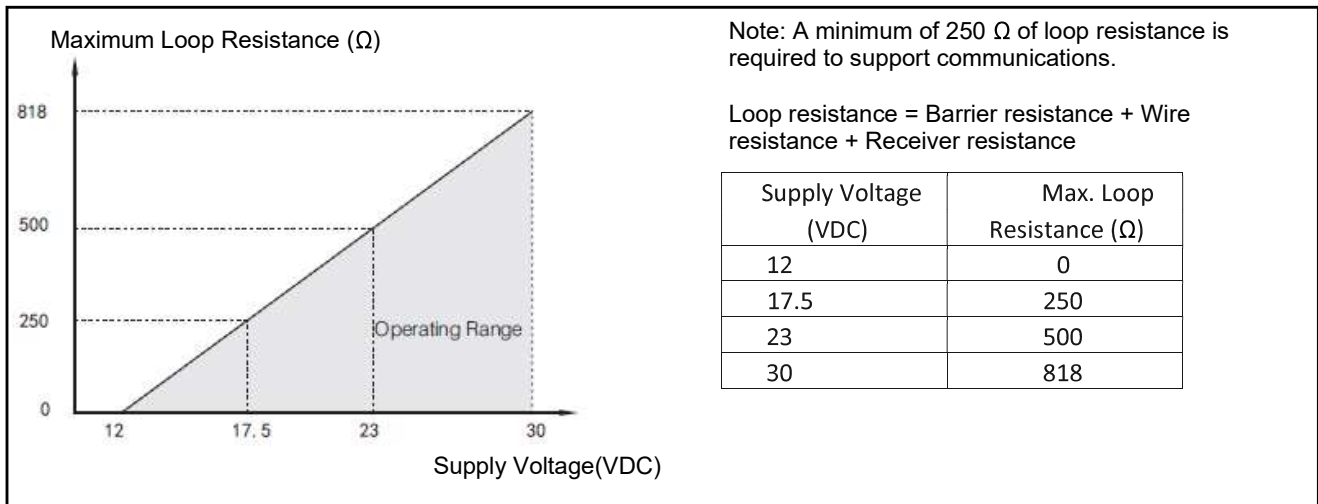
Figure 3: 2-wire load resistance
